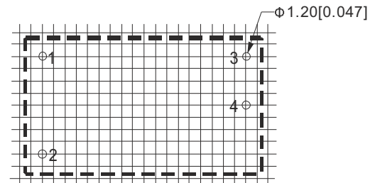
recommended PCB footprint (top view) grid: 2.54 mm (0.10 inch)
