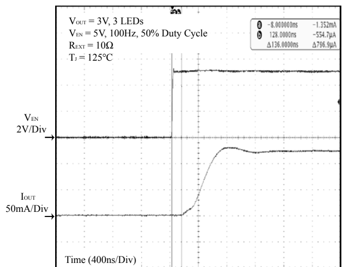
Figure 34 V_{EN} vs. I_{OUT} Delay and Rising Edge
