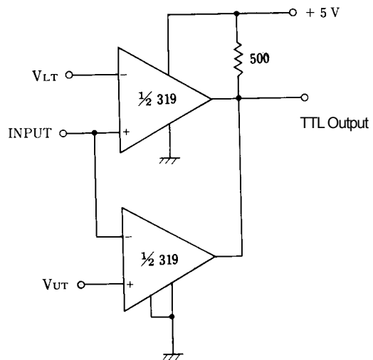
Window Detector
