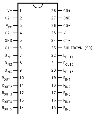
Figure 1. DS14C335 Top View See Package Number DB0028A
