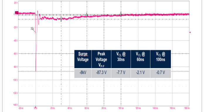
Figure 21. ESD response to IEC61000-4-2 (-8 kV contact discharge)
