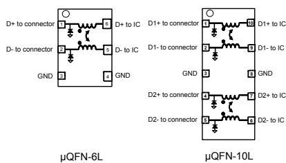
μQFN-6L
