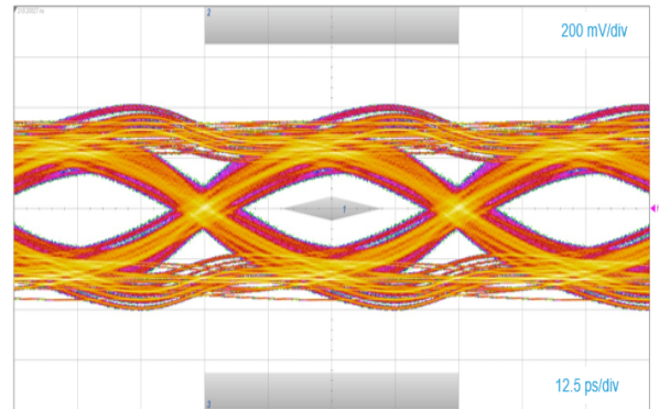
Figure 9. USB4 20.0 Gbps eye diagram with ECMFx-40A100Nx (with Preset 0, reference cable 0.8m, equalizer with ADC = 0dB and DFE)
