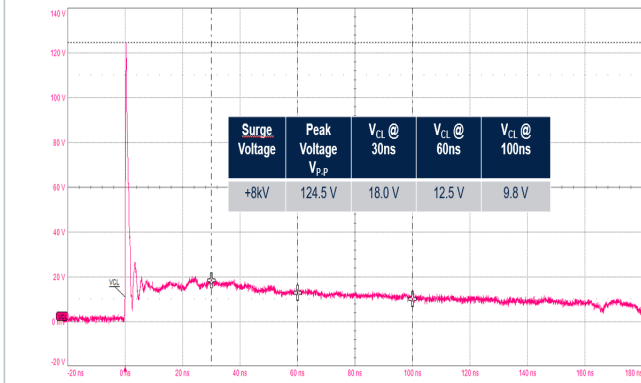
Figure 20. ESD response to IEC61000-4-2 (+8 kV contact discharge)
