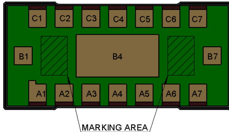
Figure 27. Product marking area
