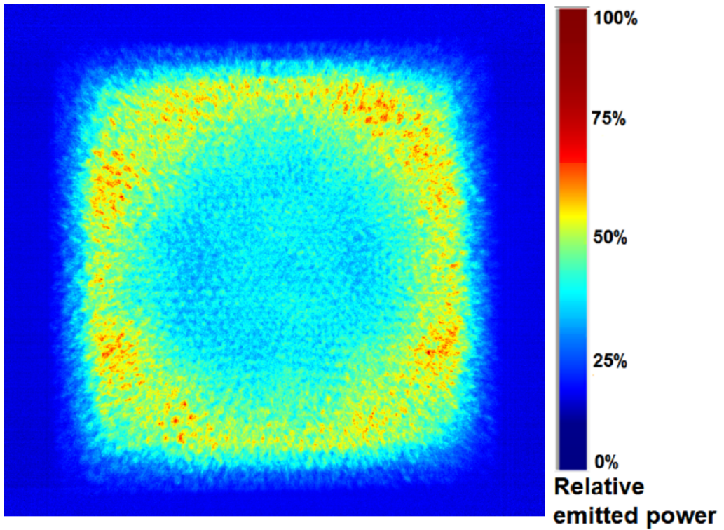
Figure 2. VL53L7CX Fol
