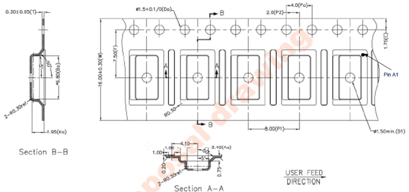
Figure 29. VL53L7CX tape outline and reel packaging drawing
