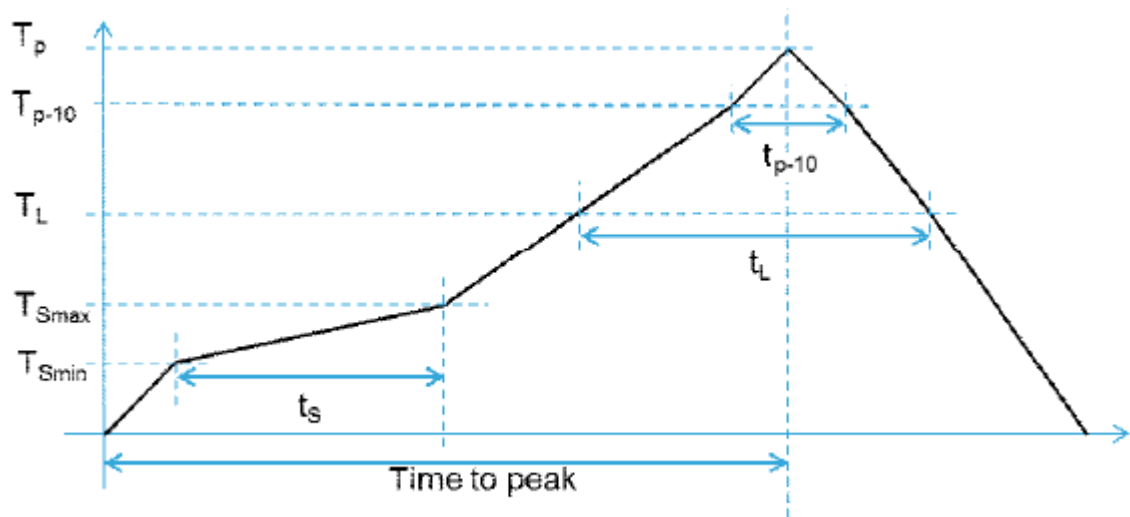
Figure 30. Solder profile
