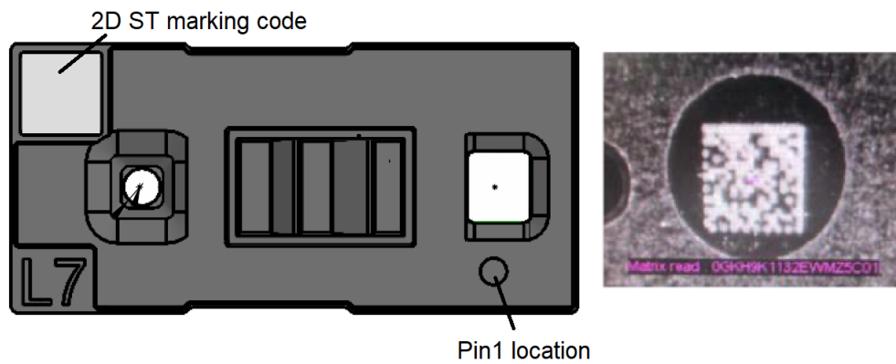
Figure 28. 2D product marking code
