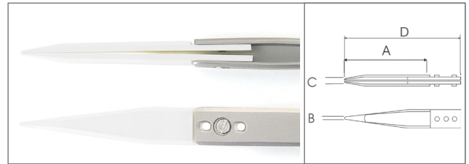
74MZ.SA A 1.6" 40 mm - B 0.04" 1.0 mm - C 0.04" 1.0 mm - D 2.2" 55 mm _ Replaceable tips set code: A74MZ
