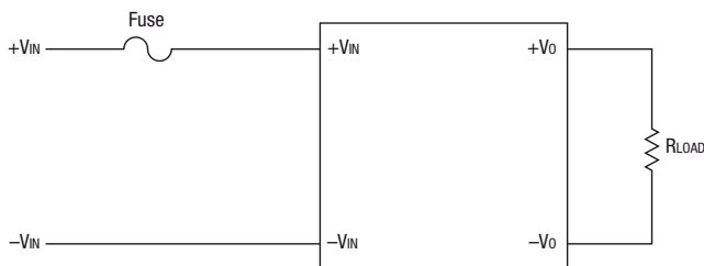
Figure 4. Input Fusing
