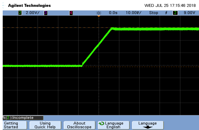
Figure 24. Output Pre-bias start-up Vin=48V, Iout = 0A, Cload = 47µF, Ta = 25°C, Pre-bias Voltage = 9.6V
