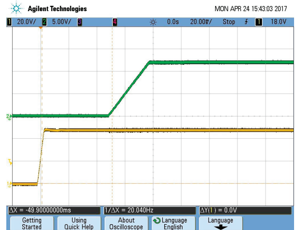
Figure 12. Vin Start-up Delay (CH2: Vout, CH1: Vin) (Vin=48V, Iout=50A, Cload=330μF, Ta=+25°C, 20ms/div)
