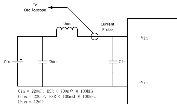
Figure 14. Measuring Input Ripple Current
