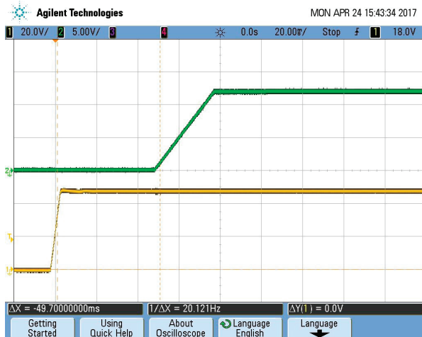
Figure 11. Vin Start-up Delay (CH2: Vout, CH1: Vin) (Vin=48V, Iout=0A, Cload=330μF, Ta=+25°C, 20ms/div)
