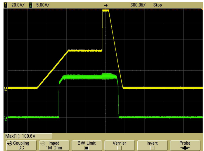
Figure 4. Test Waveform with Feedback Loop Open
