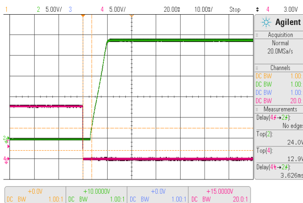
On/Off Enable Delay (Negative logic, Vin=48V, Vout=nom., Iout=2A, Cload=0 μF, Ta=+25°C., ScopeBW=20MHz) Trace 2=Enable, Trace 4=Vout
