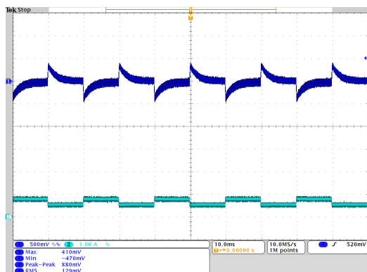
Step Load Transient Response (Vin=48V, Vout=nom., Iout=50-75-50% of full load, Cload=1μF ceramic || 10μF tantalum, Ta=+25°C., ScopeBW=20MHz)
