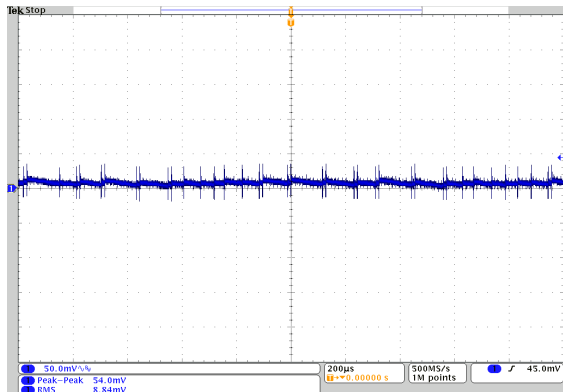
Output Ripple and Noise (Vin=48V, Vout=nom., Iout=no load, Cload=1μF ceramic || 10μF tantalum, Ta=+25°C., ScopeBW=20MHz)
