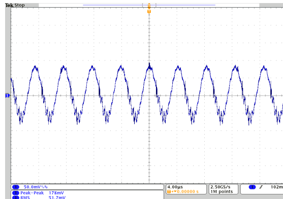
Output Ripple and Noise (Vin=48V, Vout=nom., Iout=1A, Cload=1μF ceramic || 10μF tantalum, Ta=+25°C., ScopeBW=20MHz)
