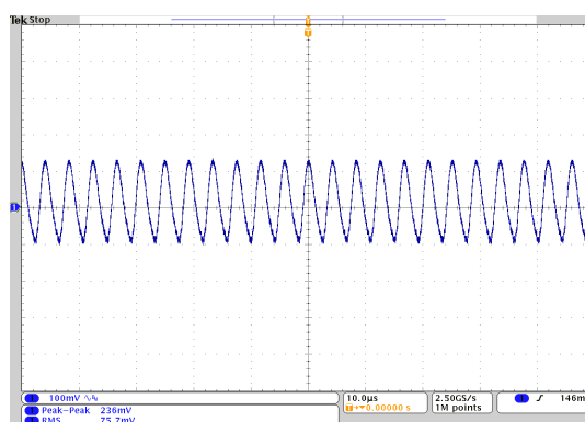
Output Ripple and Noise (Vin=48V, Vout=nom., Iout=2A, Cload=1μF ceramic II 10μF tantalum, Ta=+25°C., ScopeBW=20MHz)
