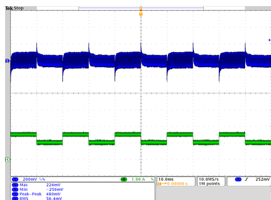
Step Load Transient Response (Vin=48V, Vout=nom., Iout=50-75-50% of full load, Cload=1μF ceramic II 10μF tantalum, Ta=+25°C., ScopeBW=20MHz)
