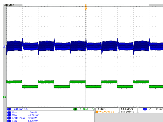
Step Load Transient Response (Vin=48V, Vout=nom., Iout=50-75-50% of full load, Cload=680μF, Ta=+25°C., ScopeBW=20MHz)
