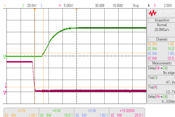
On/Off Enable Delay (Negative logic, Vin=48V, Vout=nom., Iout=1A, Cload=0 μF, Ta=+25°C., ScopeBW=20MHz) Trace 2=Enable, Trace 4=Vout
