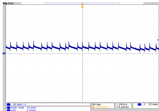
Output Ripple and Noise (Vin=48V, Vout=nom., Iout=no load, Cload=1μF ceramic II 10μF tantalum, Ta=+25°C., ScopeBW=20MHz)
