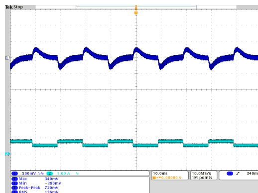
Step Load Transient Response (Vin=48V, Vout=nom., Iout=50-75-50% of full load, Cload=330μF, Ta=+25°C., ScopeBW=20MHz)
