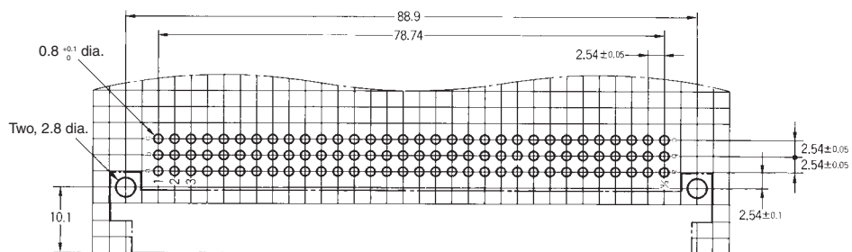
Mounting holes (bottom view)
