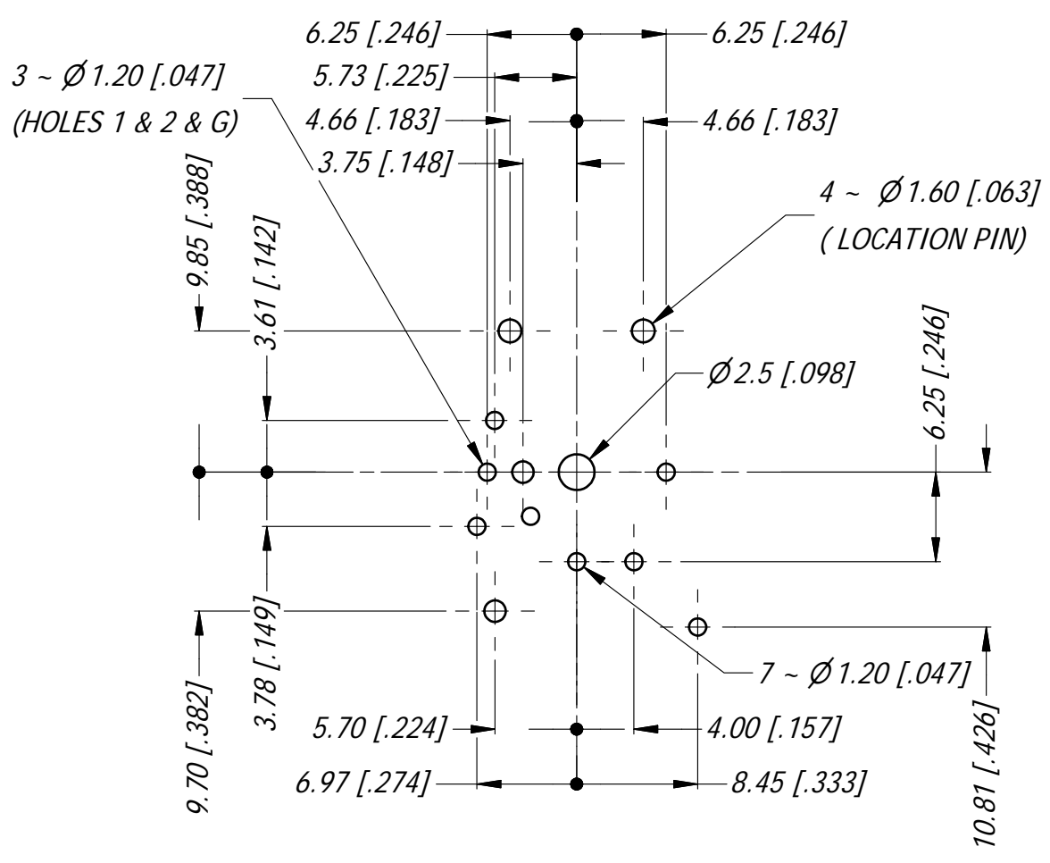
PCB LAYOUT SCALE 3:2
