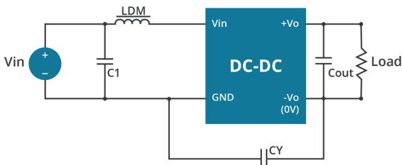
Dual Outputs
