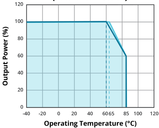
TEMPERATURE DERATING CURVE \pm 5 Vdc output (natural convection)
