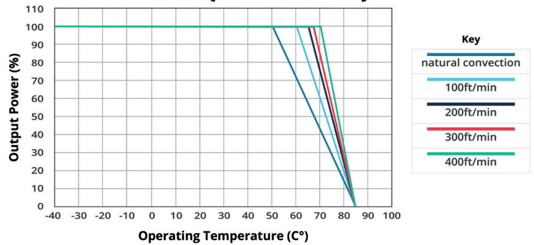
TEMPERATURE DERATING CURVE heatsink version (Vin = 115 V & 230 V)
