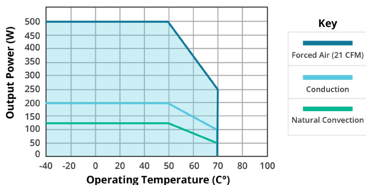
TEMPERATURE DERATING CURVE (12 & 15 Vdc output models)
