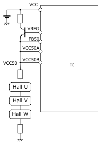
Figure 9. The Reference voltage circuit using external NPN transistor
