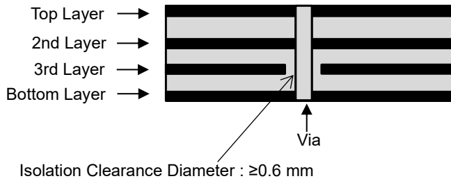
Cross Section
