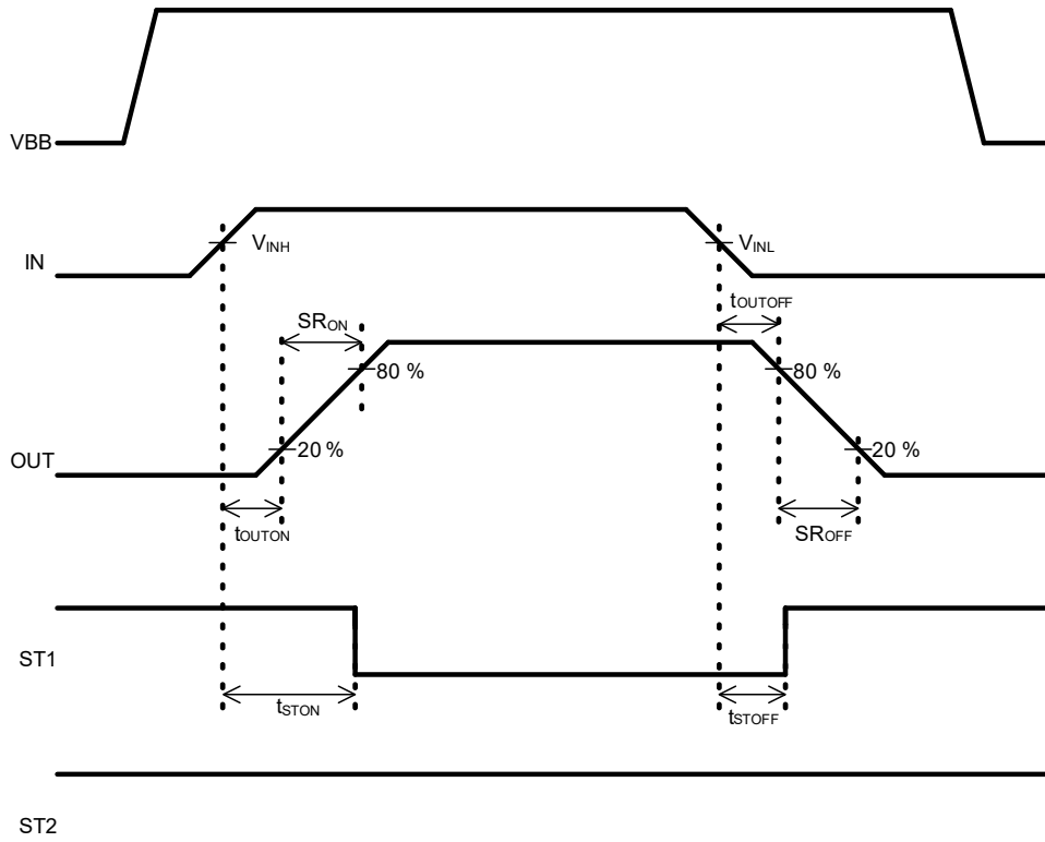
Figure 33. Timing Chart
