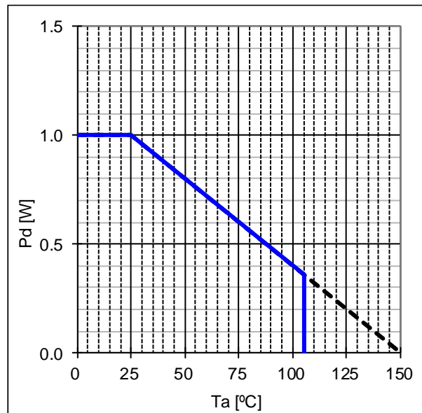
Figure 14. DIP7K Thermal Dissipation Characteristic
