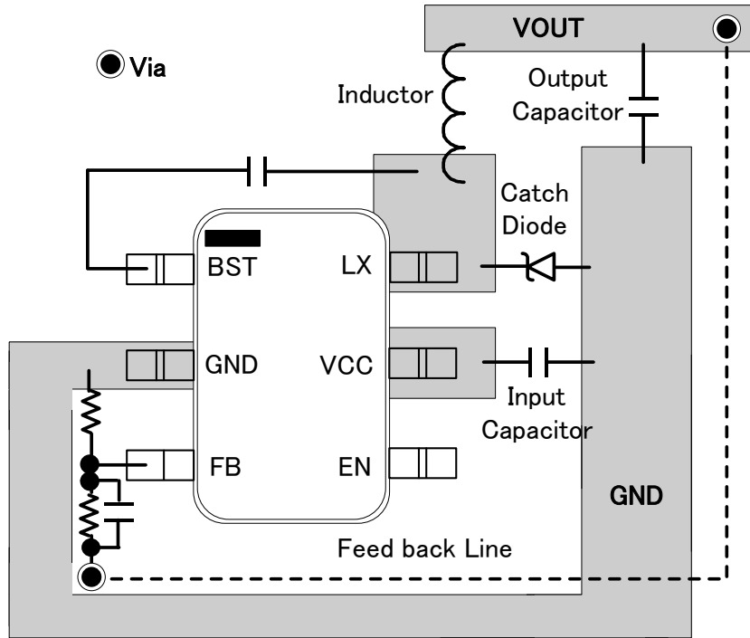
Figure 45. Reference PCB
