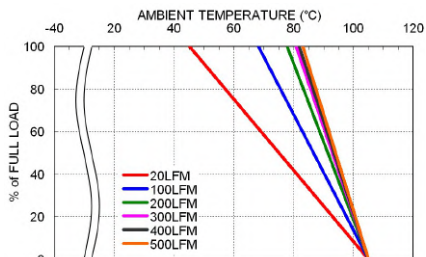
FED60-48S12W Derating Curve
