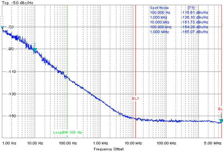
M100V-019.2MHz Typical Phase Noise
