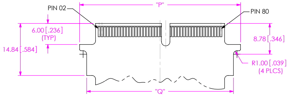
FIG 7 -40 POSITION WITH -BL OPTION SHOWN (SAME AS FIG 5, EXCEPT AS SHOWN) (FOR POSITION: -09, -13, -25, -40, -49, -50, & -60)
