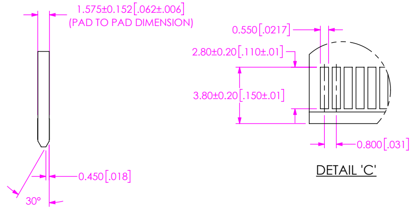
FIG 5 -40 POSITION SHOWN (FOR POSITION: -09, -13, -25, -40, -49, -50, -60, -09-L2, -13-L2, -25-L2, -49-L2)
