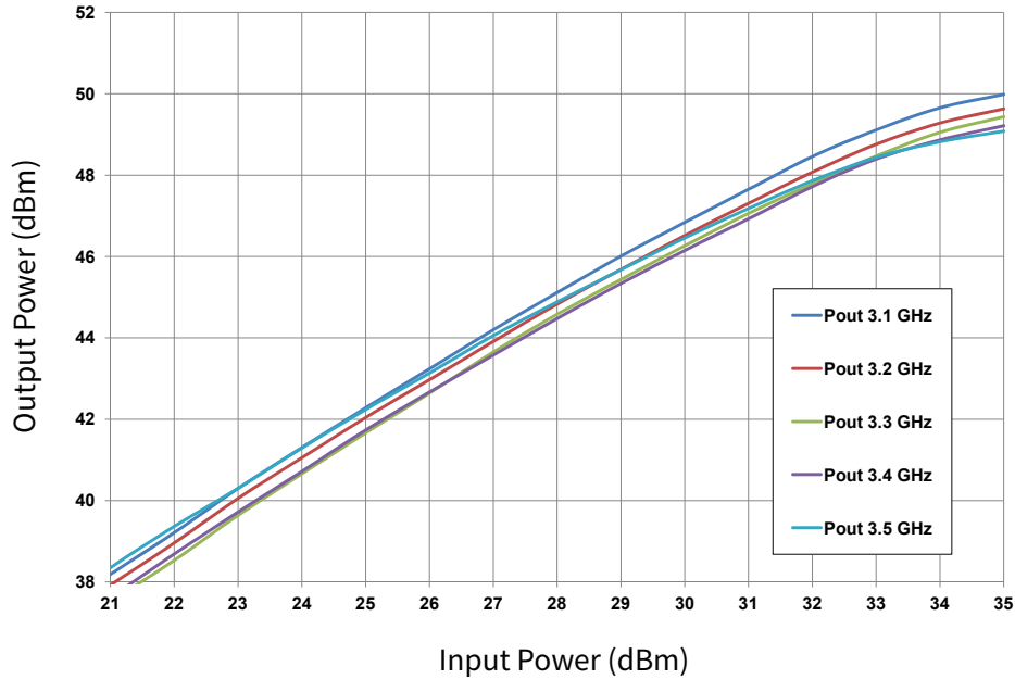
Figure 3. CGHV35060MP-AMP1 Output Power vs. Input Power V_{DD} = 50\text{ V} I_{DQ} = 125\text{ mA} , Pulse Width = 100 us, Duty Cycle = 10%, Tcase = 25°C
