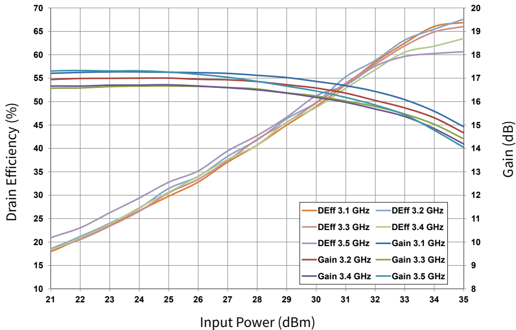
Figure 4. CGHV35060MP-AMP1 Gain & Efficiency vs Input Power V_{DD} = 50\text{ V} I_{DQ} = 125\text{ mA} , Pulse Width = 100 us, Duty Cycle = 10%, Tcase = 25°C
