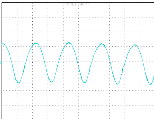
Figure 12: Output voltage ripple at nominal input voltage ( V_{in}=48V ) and rated load current (50 mV/div, 2µs/div). Load capacitance: 1µF ceramic capacitor and 10µF tantalum capacitor. Bandwidth: 20 MHz. Scope measurements should be made using a BNC cable (length shorter than 20 inches). Position the load between 51 mm to 76 mm (2 inches to 3 inches) from the module
