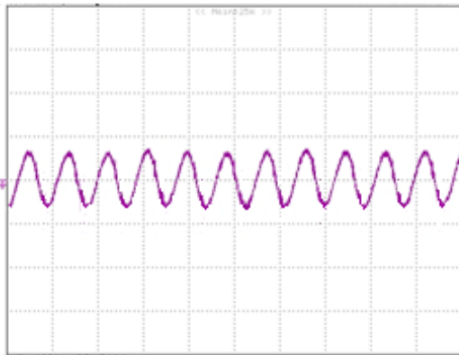
Figure 10: Input reflected ripple current, i_S , through a 12µH source inductor at nominal input voltage ( V_{in}=48V ) and rated load current (20 mA/div, 5µs/div)
