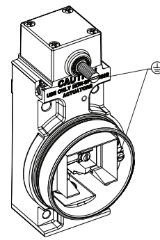
Figure 11. Wiring Instructions
