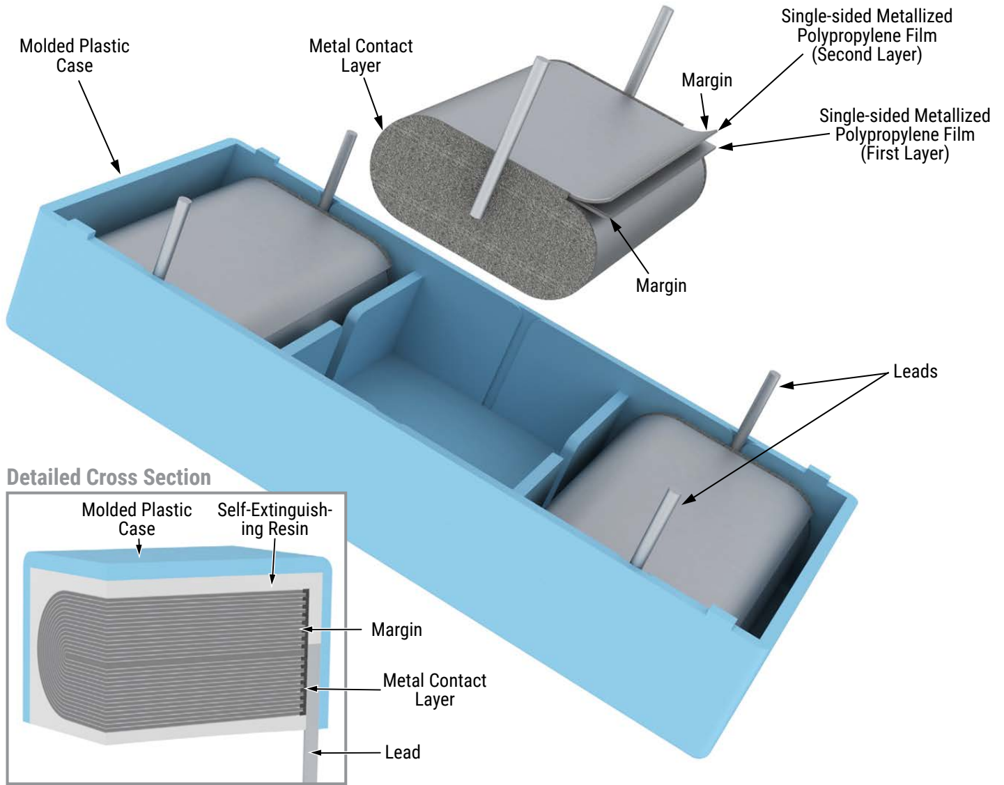
Winding Scheme
