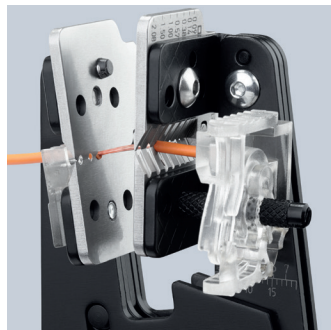
Quality stripping due to precise shape of the blades
