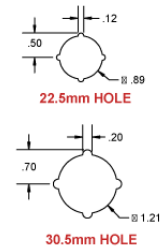
30.5mm HOLE
