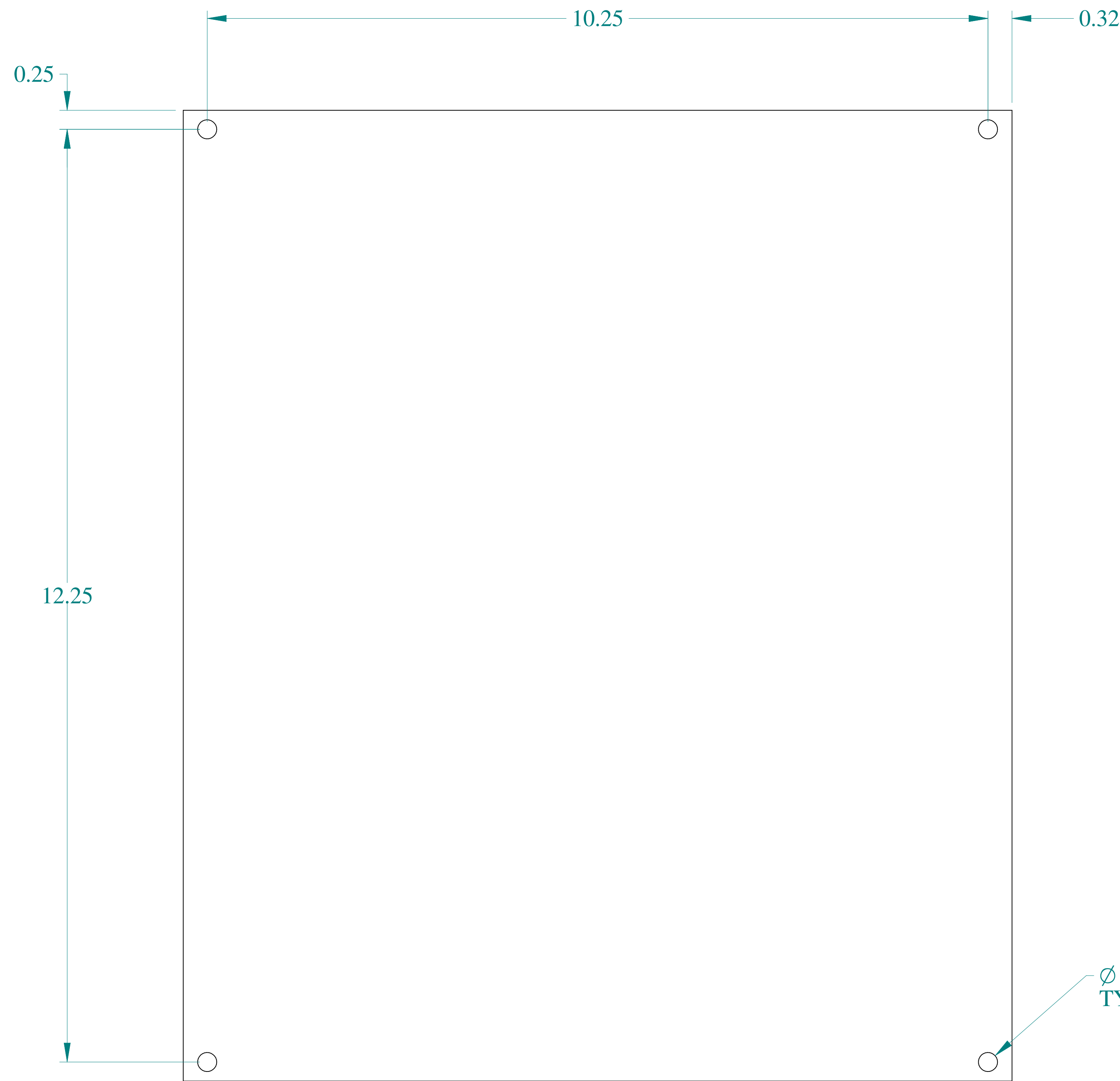
FRONT VIEW
