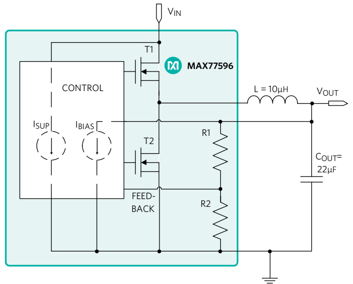
Figure 3. MAX77596 Buck Converter Fixed Output
