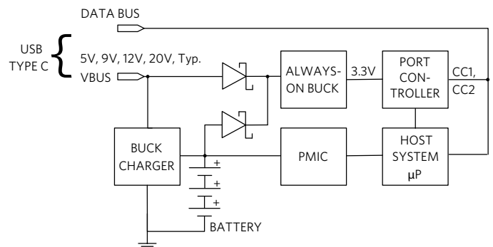
Figure 2. USB 3.1 Type C Power Management System
