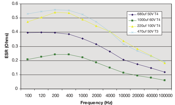
Graph 1.3.3. b TWA Frequency Dependence of ESR
