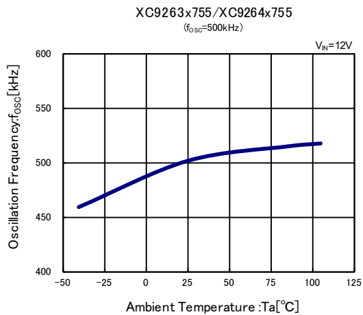
(6) Oscillation Frequency vs. Ambient Temperature
