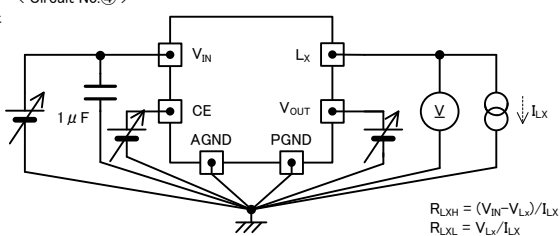
< Circuit No.④ >
