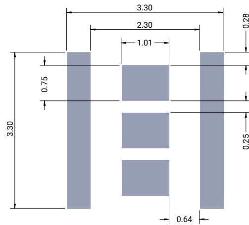
Recommended Stencil Openings*
