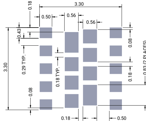
Recommended Stencil Openings*
