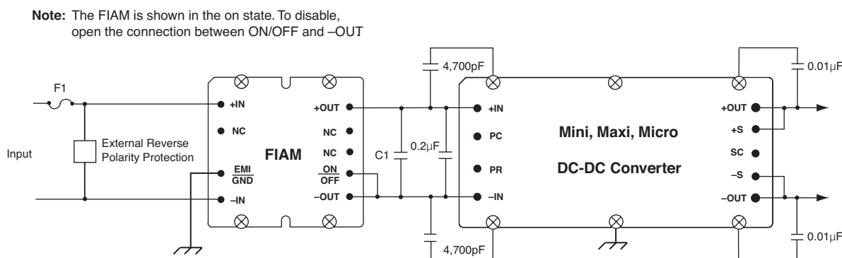
Figure 11.1 — Typical application (FIAM)
