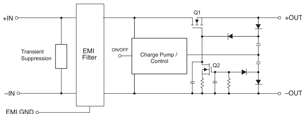
Figure 11.2 — Block diagram (FIAM)
