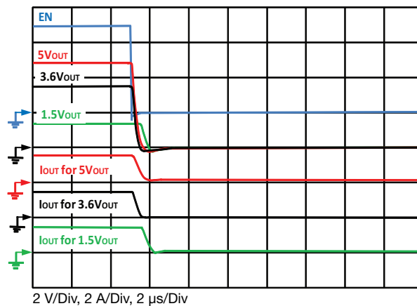
Fig. 24 - Typical Fall Time C_{OUT} = 0.1 \mu\text{F} , C_{IN} = 4.7 \mu\text{F} , I_{OUT} = 1.5 \text{ A}
