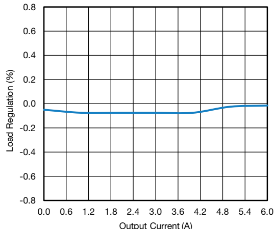
Fig. 44 - Load Regulation
