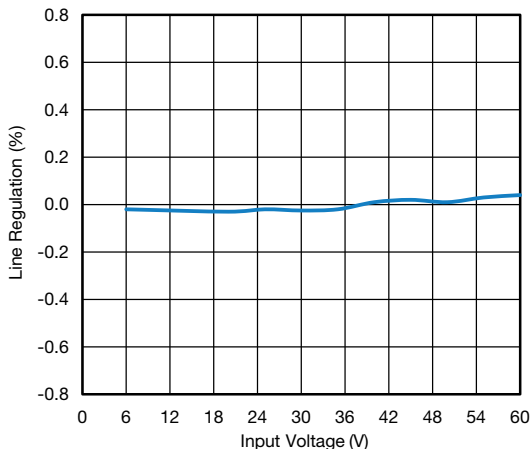
Fig. 41 - Line Regulation
