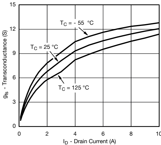
Transconductance
