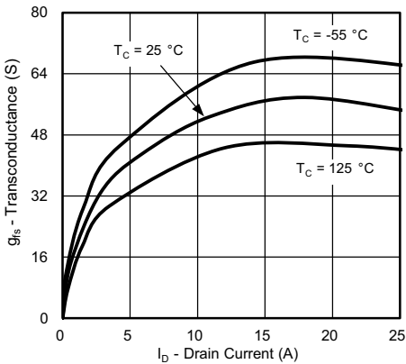
Transconductance
