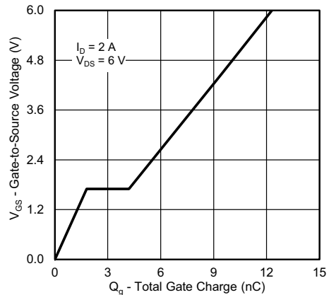
Gate Charge
