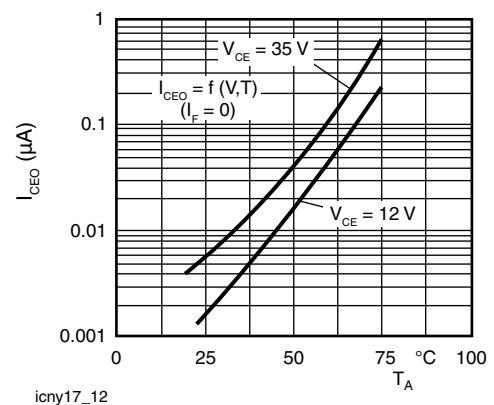
Fig. 11 - Leakage Current vs. Ambient Temperature
