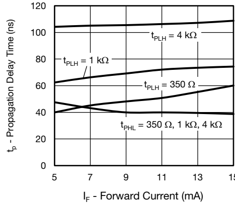
Fig. 13 - Propagation Delay Time vs. Diode Forward Current
