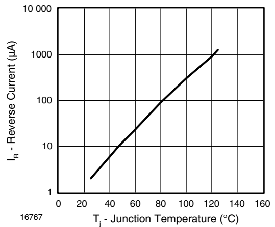
16767 Fig. 3 - Reverse Current vs. Junction Temperature
