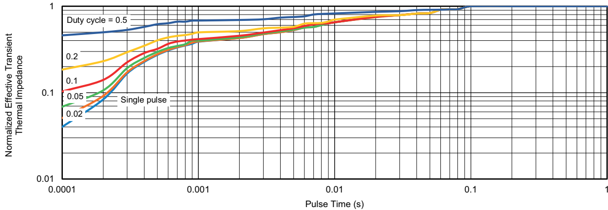
Fig. 12 - Normalized Thermal Transient Impedance, Junction-to-Case
