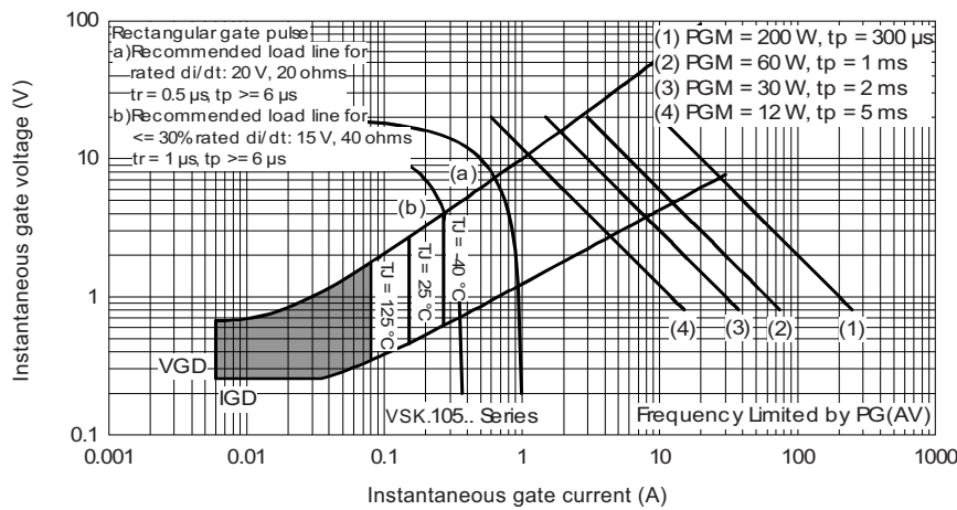
Fig. 12 - Gate Characteristics
