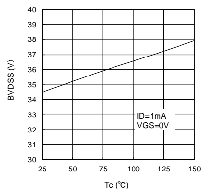
BVDS-Tc characteristics (typical)
